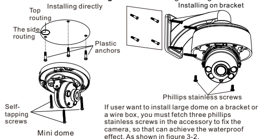
Figure 3-2 Installing housing
